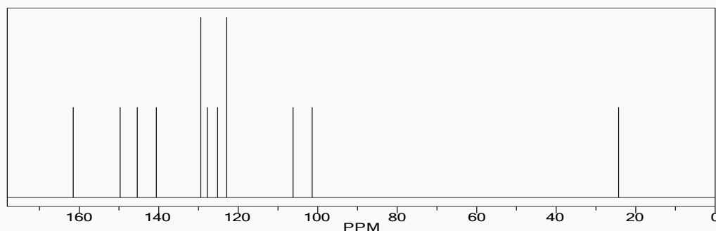
4-rasm. 6-metilpiridel-2-azo-m-aminofenol molekulasiyning ChemOffice dasturi yordamida olingan YaMR- \text{C}^{13} spektri.
