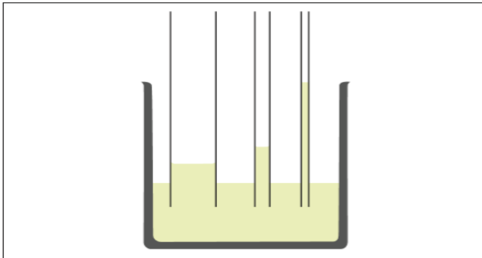
1.3-rasm Stakandagi rangli suv ichidagi to'g'ri kapillyar naychalar
