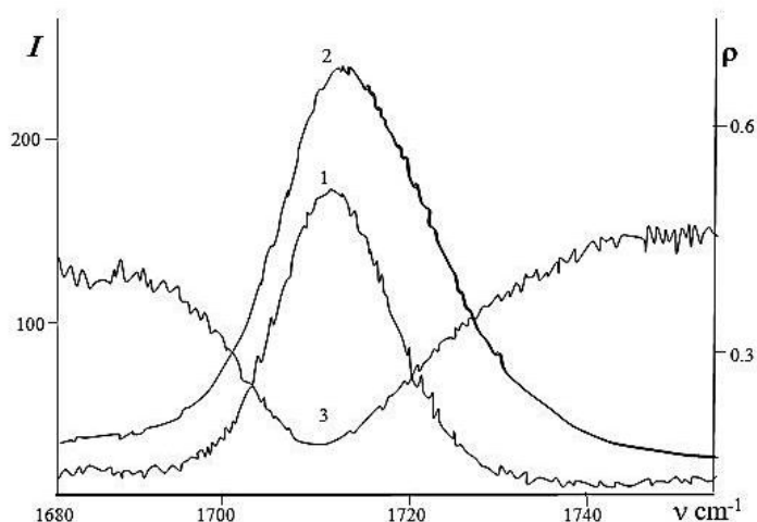
1-rasm. Toza MEK suyuqligining C=O valent tebranishiga tegishli kombinatsion sochilish spektrlari: 1) I_{\perp} parallel tashkil etuvchi; 2) I_{\parallel} parallel tashlik etuvchisi; 3) dipolyarizatsiya koeffitsienti ( \rho = I_{\perp}(\nu) / I_{\parallel}(\nu) ).
