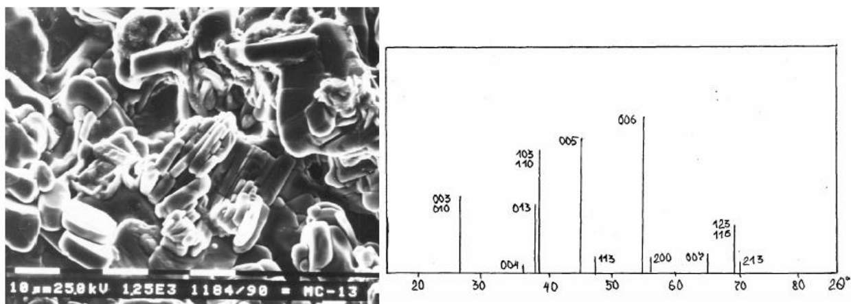
Fig. 2. SEM image of textured BTCII ceramics 1 2 3 sintered from YДП after pre-loaded during pressing and barcode diagram of X-ray phase analysis ((CoK \alpha radiation)
